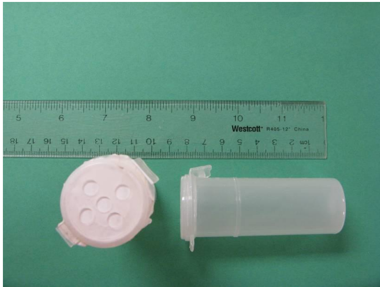
Figure 10. Peeper-style passive samplers used to collect porewater samples from Ballona Creek Estuary for trace metal measurement.
