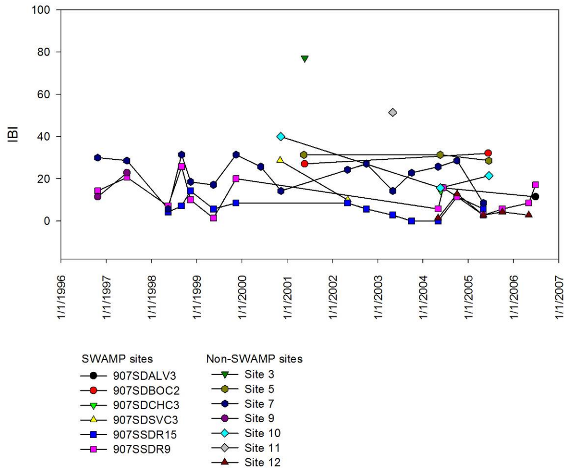
Figure 12. IBI values for each year and site. Each symbol represents a single sample.
