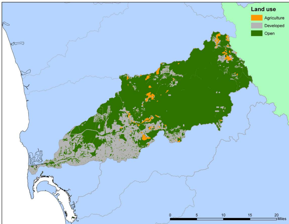
Figure 4. Land use within the San Diego HU. Undeveloped open space is shown as green. Agricultural areas are shown as orange. Urban and developed lands are shown as dark gray.
