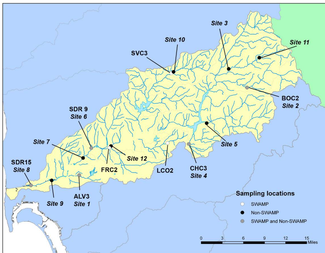
Figure 5. Sampling locations in the San Diego HU. White circles represent sites sampled under SWAMP. Black circles represent sites sampled under non-SWAMP programs. Gray circles represent sites sampled under both SWAMP and non-SWAMP programs. The SWAMP site prefix designating the hydrologic unit (i.e., 907SD-) has been dropped to improve clarity.
