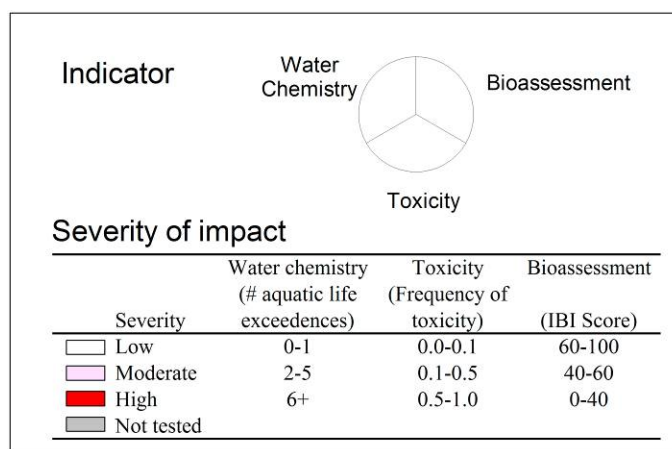
Figure 14. Summary of the ecological health of SWAMP sites in the San Diego HU, as determined by water chemistry, toxicity, and bioassessment indicators. Each pie slice corresponds to a specific indicator, as described in the inset, with darker colors corresponding to more degraded conditions (unmeasured indicators are shown in cross-hatched gray). The top-left slice corresponds to the number of water chemistry constituents exceeding aquatic life thresholds. The bottom slice corresponds to the frequency of toxicity among three endpoints: C. dubia (fecundity), H. azteca (growth), and S. capricornutum (total cell count). The top-right slice corresponds to the IBI of bioassessment samples.
