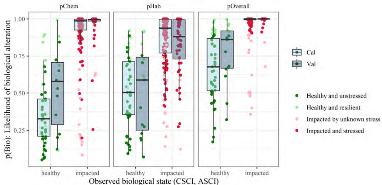
Figure 5. Boxplot distributions of the modelled likelihood of biological alteration relative to water chemistry ( pChem , eqn. (1)) and physical habitat variables ( pHab , eqn. (2)) and the additive overall stress as the product between the two ( pOverall , eqn. (3)). Groups are separated into healthy or impacted biological condition at each site (Table 1) as the response measure for each model and by calibration/validation datasets (3:1 split). Model precision can be evaluated by comparing the differences between the boxplots for the validation data for healthy and impacted categories, whereas model bias can be assessed by comparing the distributions between calibration and validation data among biological state and models. Points show the four possible categorical outcomes from the overall SQI. CSCI: California Stream Condition Index, ASCI: Algal Stream Condition Index.
