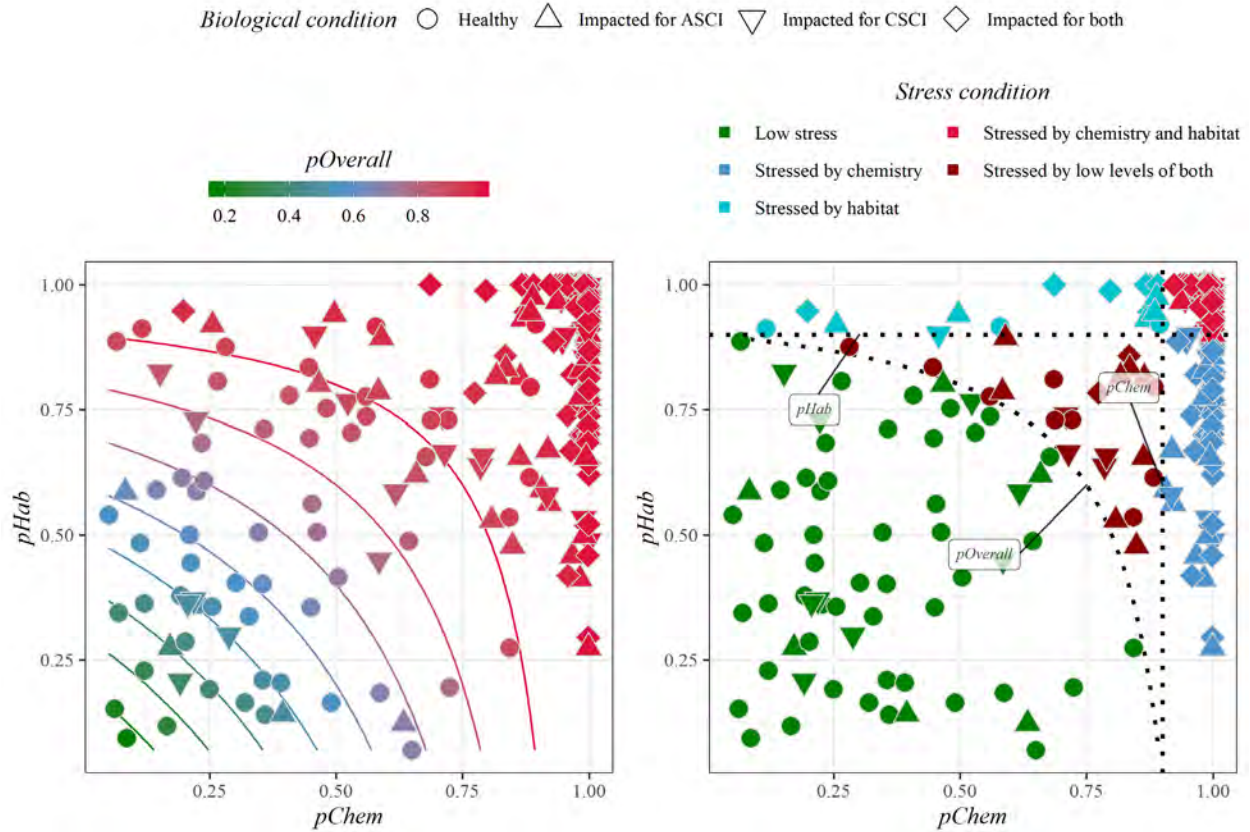
Figure 6. Relationship between stress models for water chemistry ( p_{Chem} , eqn. (1)) and physical habitat ( p_{Hab} , eqn. (2)). Stress models for water chemistry and physical habitat were created based on the likelihood of biological alteration for the observed stress measures. The overall stress measures ( p_{Overall} , eqn. (3)) is the product of both stress models shown in the left plot. Points represent estimated stress at a single site, with shapes showing the biological condition. The right plot shows the same points but colored by the stress condition categories that are defined by thresholds from the dotted lines.
