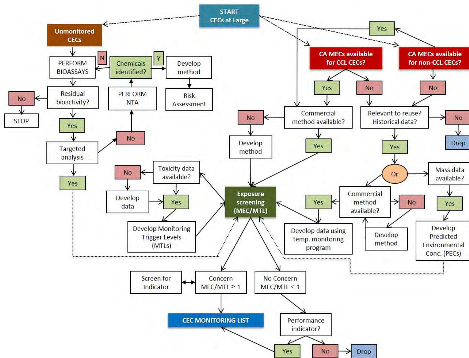
Figure 5.1. Revised risk-based CEC selection framework.
