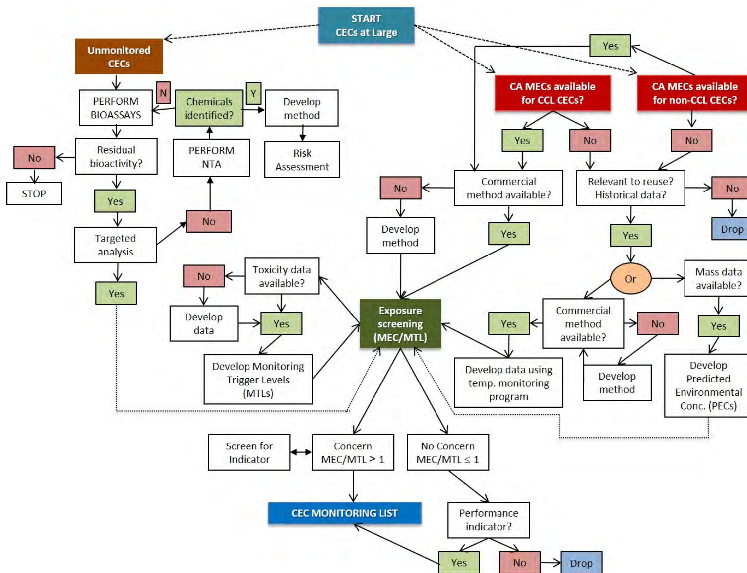
Figure ES.1. Revised risk-based CEC selection framework.
