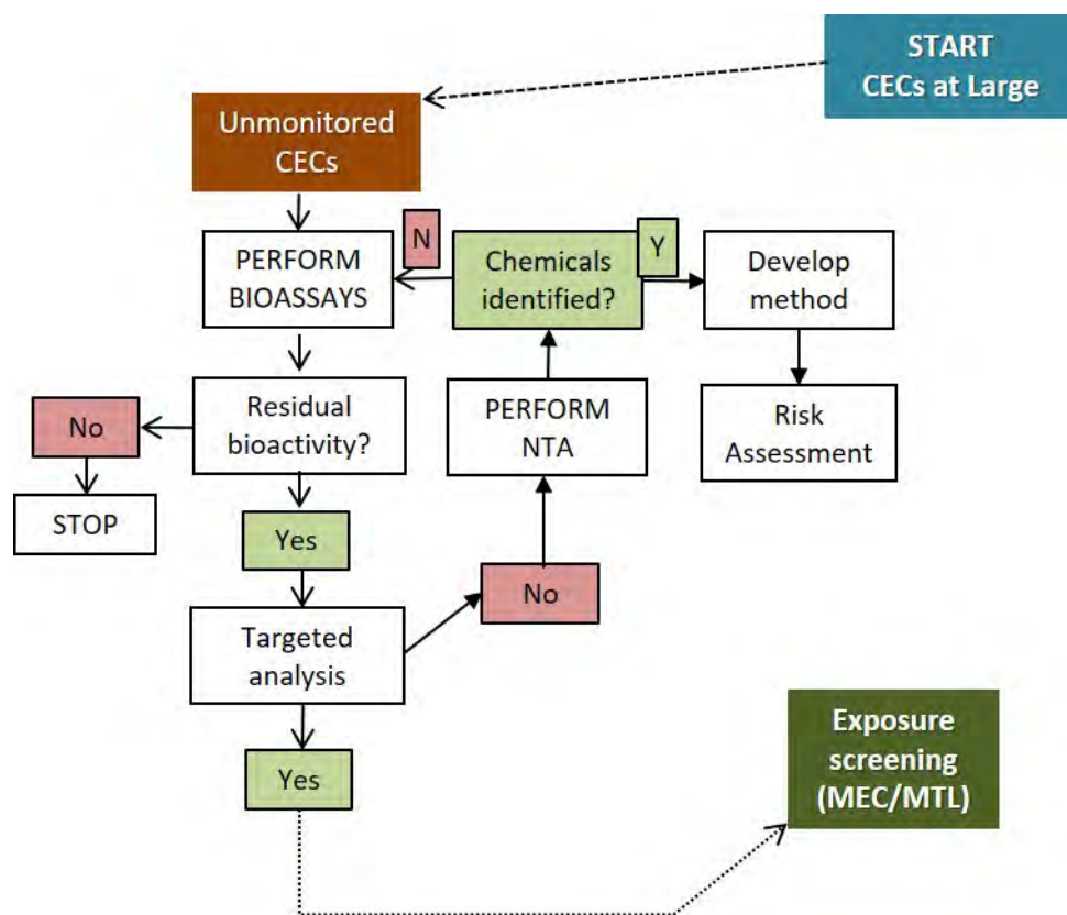
Figure 7.1. Screening approach for unmonitored CECs using bioanalytical tools and non-targeted chemical analysis (NTA) in recycled water.
