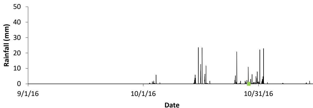
Figure D-6. Rainfall at Ukiah Airport. Green points represent the approximate timing of water sample collection at the Potter Valley and Hopland sites, which are in the vicinity of the NOAA Ukiah Municipal Airport rain gauge station (Station ID 72590523275).
