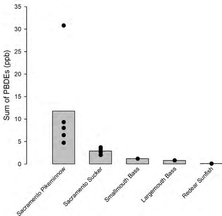
Figure 2-2. Sums of PBDE concentrations (ppb wet weight) in sport fish species in the Russian River watershed, 2015. Bars indicate average concentrations. Points represent composite samples of fillets without skin. All samples were well below the lowest OEHHHA threshold (the 100 ppb 2-serving ATL).
