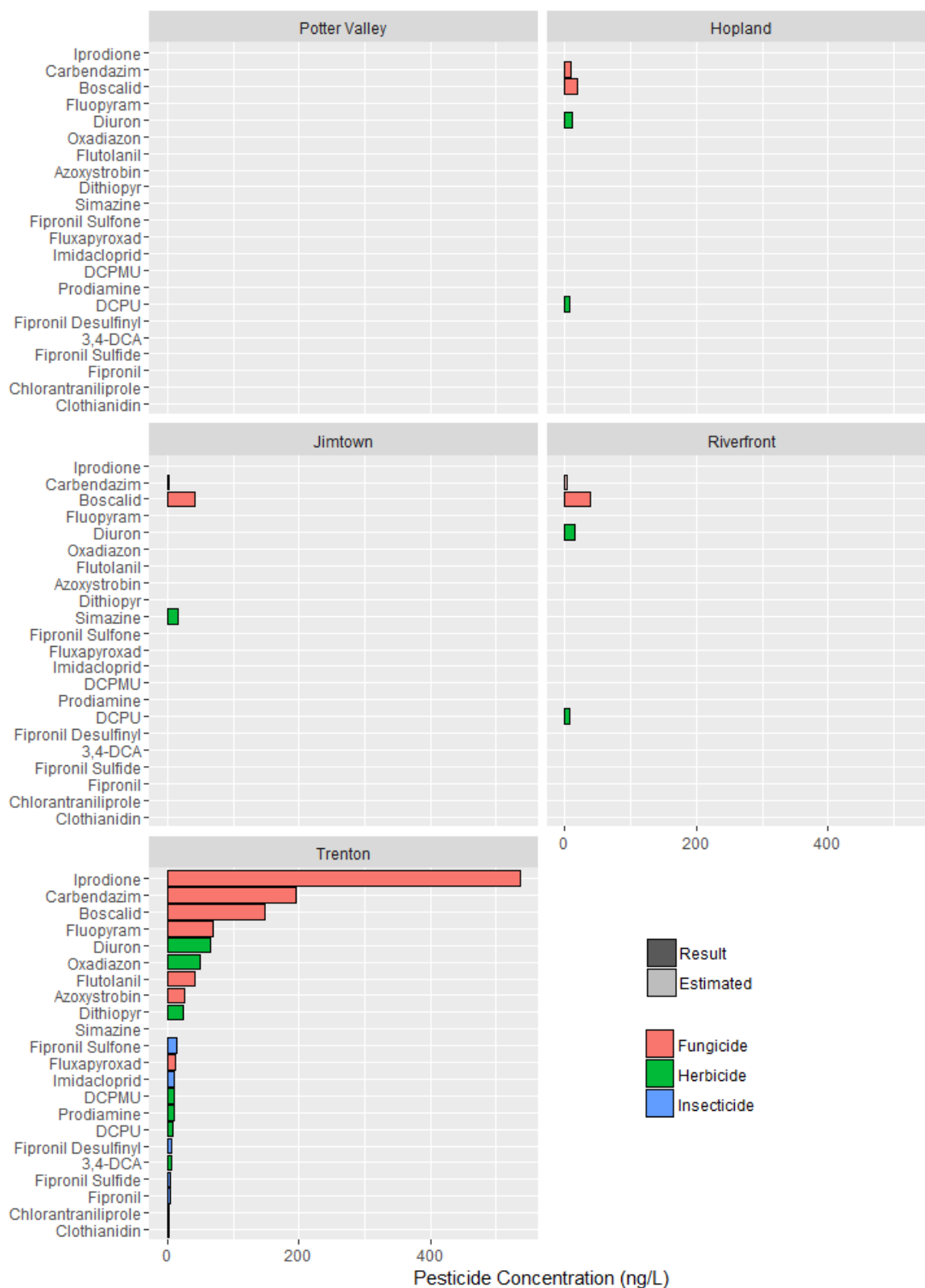
Figure 3-2. Water results by location – detected analytes
