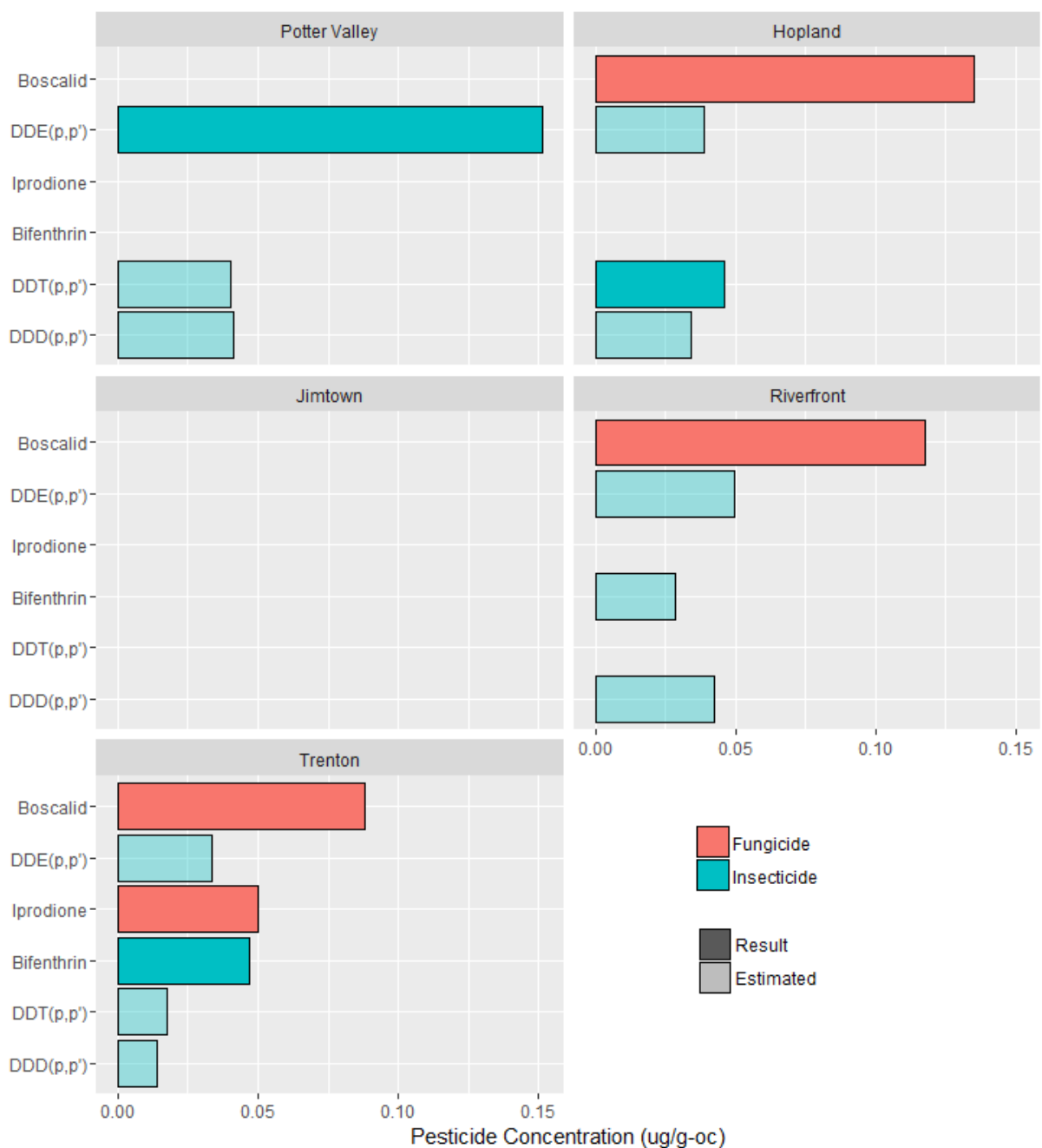
Figure 3-4B. Sediment results ( \mu\text{g/g-oc} ) by location – detected analytes
