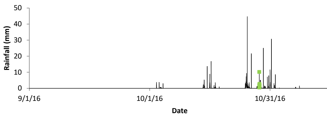
Figure D-7. Rainfall at Sonoma Airport. Green points represent the approximate timing of water sample collection at the Jintown, Riverfront, and Trenton Road sites, which are in the vicinity of the NOAA Sonoma County Airport rain gauge station (Station ID 74295723213).
