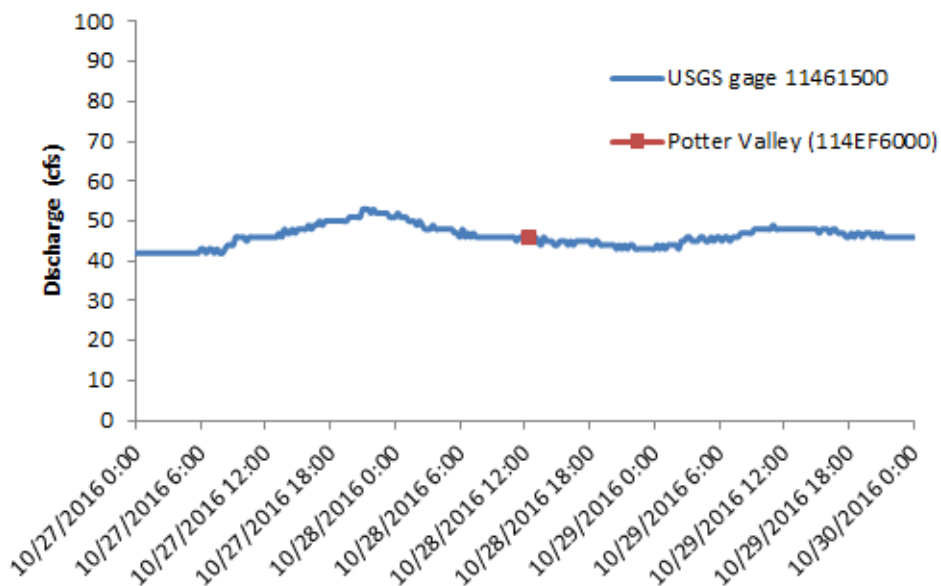
Figure B-2A. Storm hydrograph near the Potter Valley sampling site
