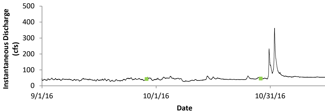
Figure D-2. Hydrograph measured at the Hopland site. Data from USGS stream gauge 11462500. Green dots represent sampling dates for sediment (September) and water (October).
