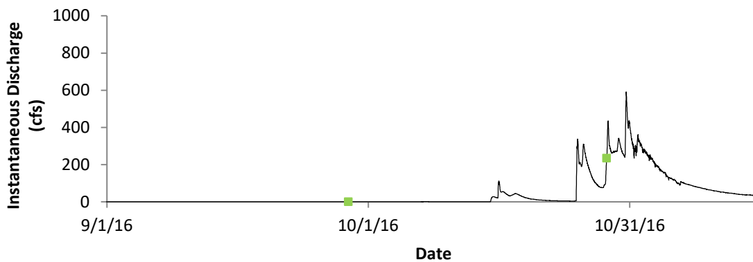
Figure D-5. Hydrograph at the Trenton Road site. Data from USGS stream gauge 11466800. Green dots represent sampling dates for sediment (September) and water (October).
