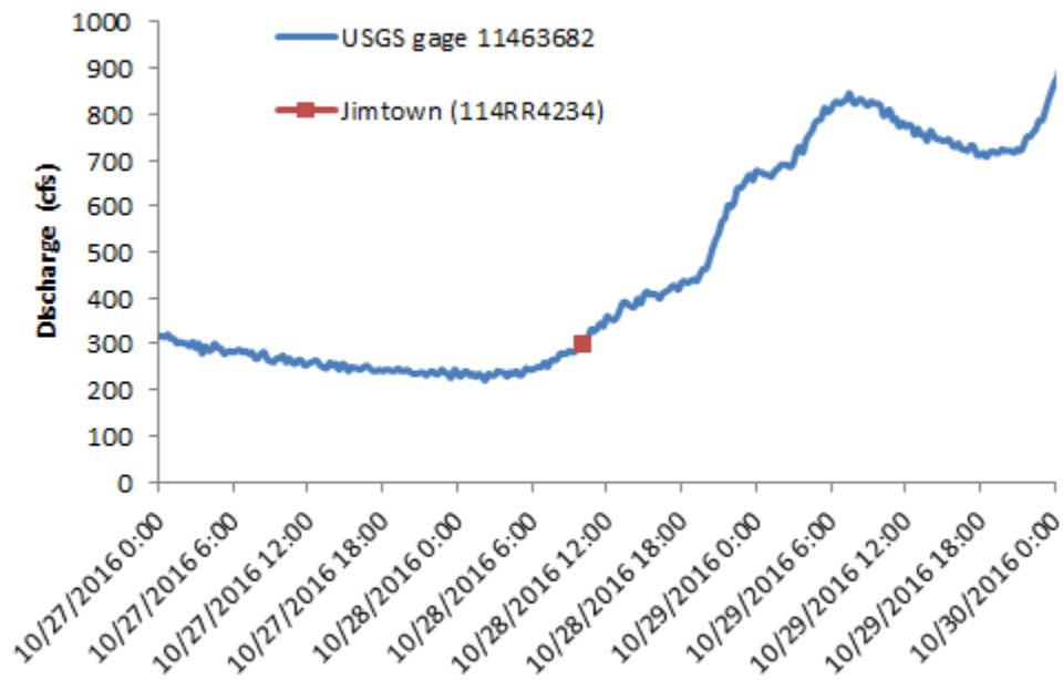
Figure B-2C. Storm hydrograph at the Jimtown sampling site
