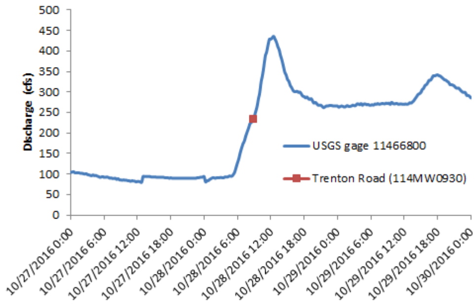
Figure B-2E. Storm hydrographs near the Trenton Road sampling site
