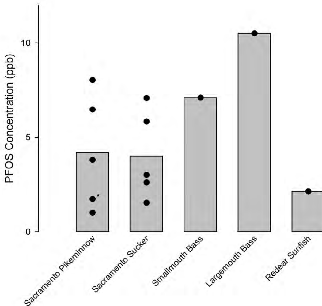
Figure 2-4. PFOS concentrations (ppb wet weight) in sport fish species in the Russian River Watershed, 2015. Bars indicate average concentrations. Points represent composites, except for one of the pikeminnow samples (an individual fish marked with an asterisk). All samples were well below the lowest MDH meal advice category (no more than one meal per week if PFOS > 40 – 200 ppb).
