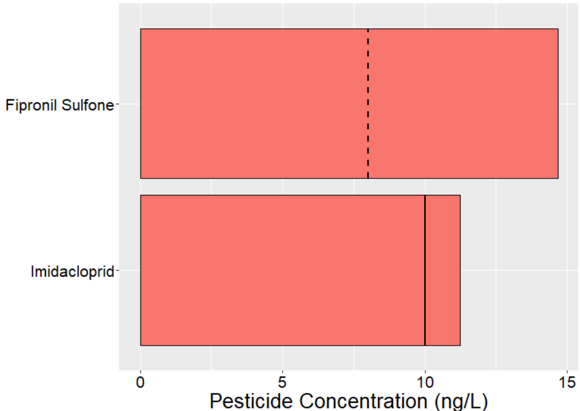
Figure 3-3. Water results that exceed toxicity thresholds. All values shown were measured at the mixed-use Trenton Road site. The solid line represents an Environmental Protection Agency, Office of Pesticide Protection chronic aquatic invertebrate benchmark (imidacloprid=10 ng/L). The dashed line represents chronic aquatic invertebrate toxicity thresholds that have not been formalized into an EPA OPP benchmark. This threshold for fipronil sulfone was established by Weston & Lydy 2014 (Fipronil sulfone=8 ng/L).
