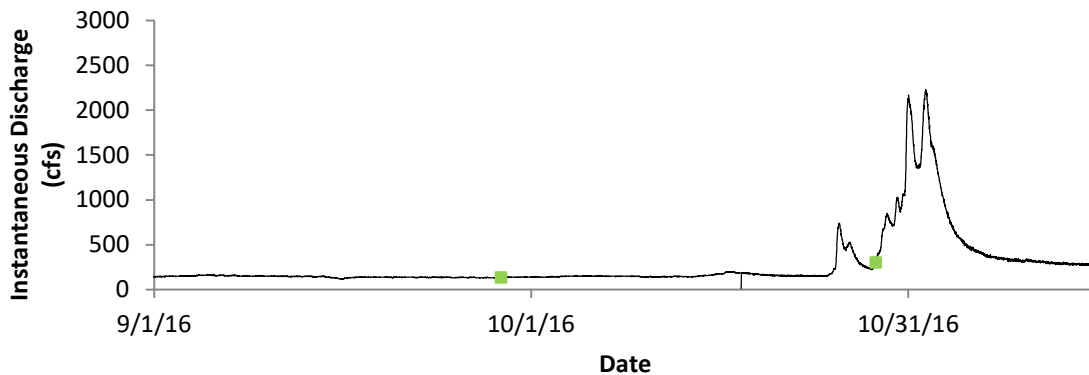
Figure D-3. Hydrograph at the Jimtown site. Data from USGS stream gauge 11463682. Green dots represent sampling dates for sediment (September) and water (October).
