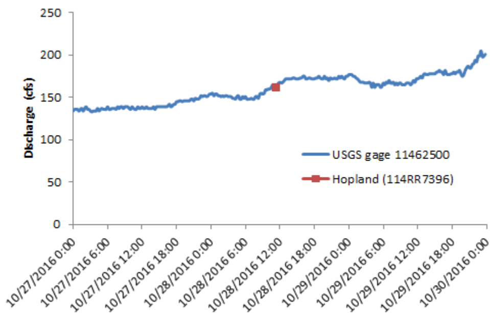
Figure B-2B. Storm hydrograph at the Hopland sampling site
