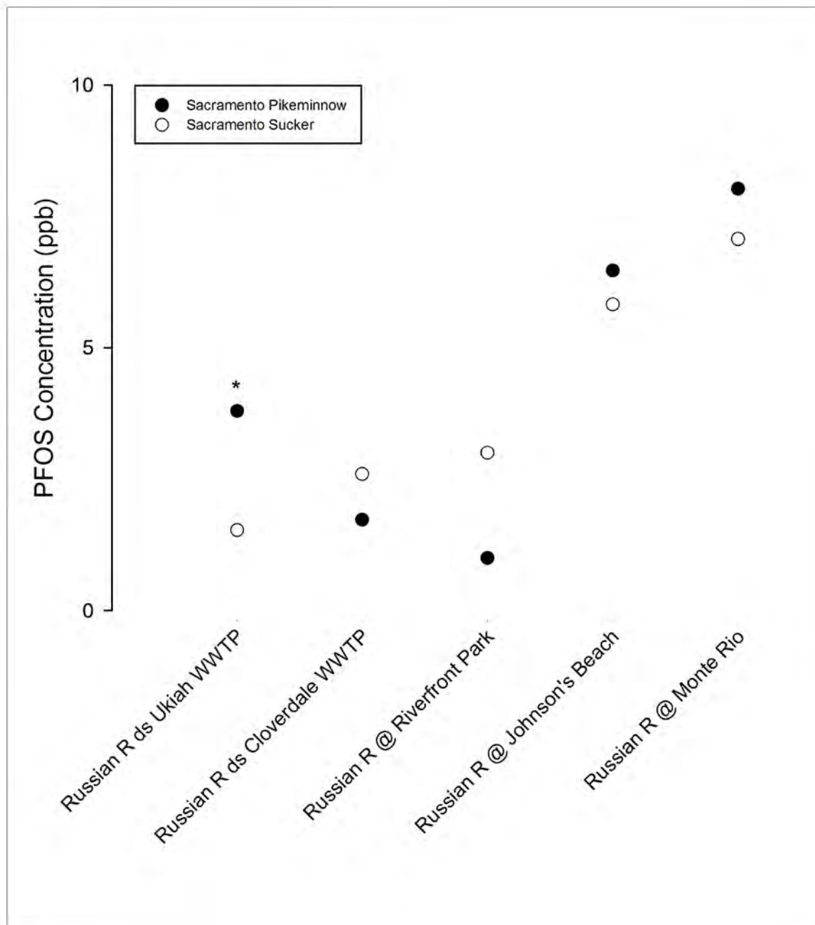
Figure 2-5. PFOS concentrations (ppb) in sport fish species collected at different locations along the Russian River watershed, 2015. Points represent results for composite samples, except for one of the Sacramento Pikeminnow samples (an individual marked with an asterisk).
