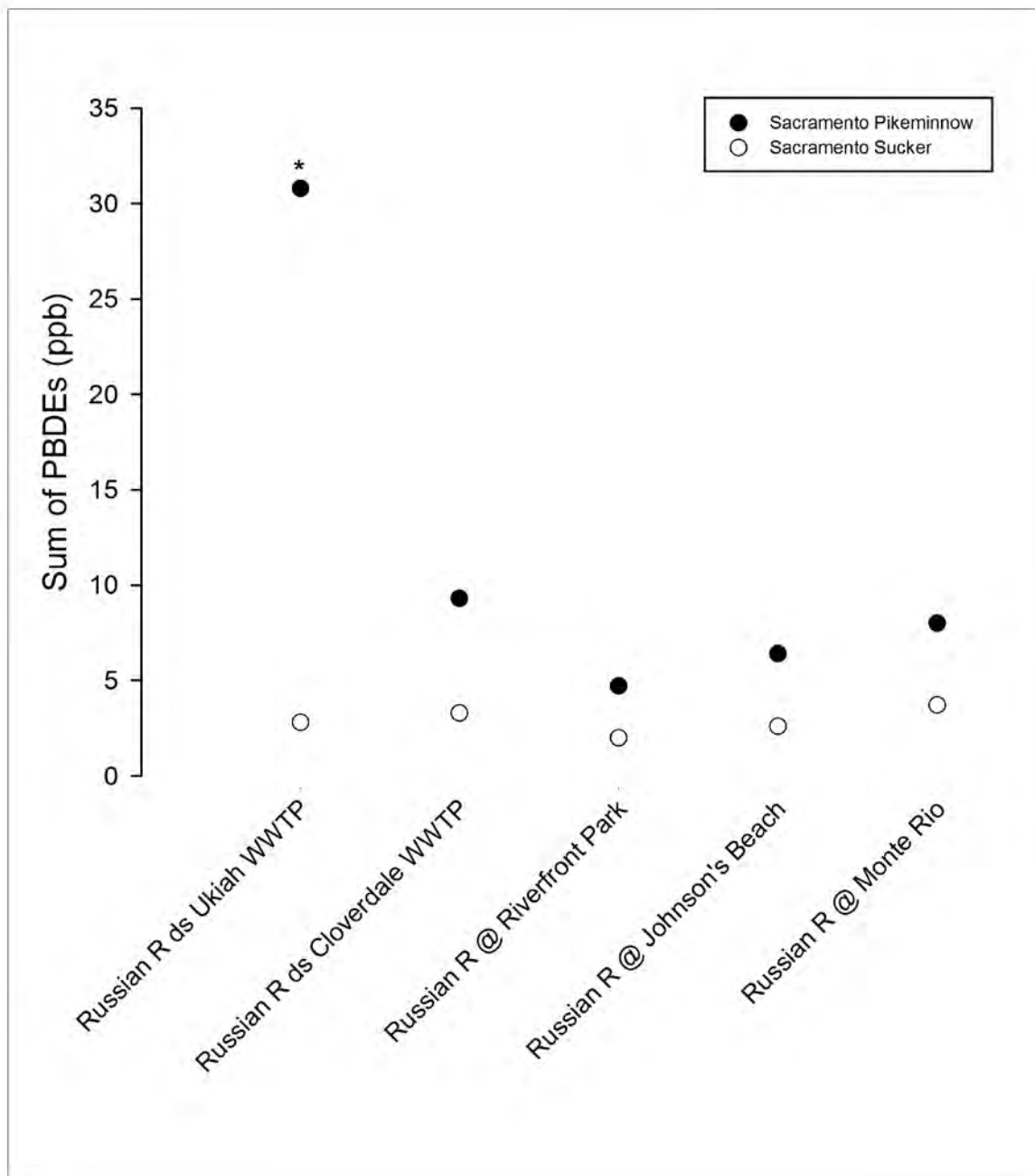
Figure 2-3. Sums of PBDE concentrations (ppb wet weight) in sport fish collected at different locations along the Russian River watershed, 2015. All points represent composites, except for one of the Sacramento Pikeminnow samples that was an individual fish (marked with an asterisk).
