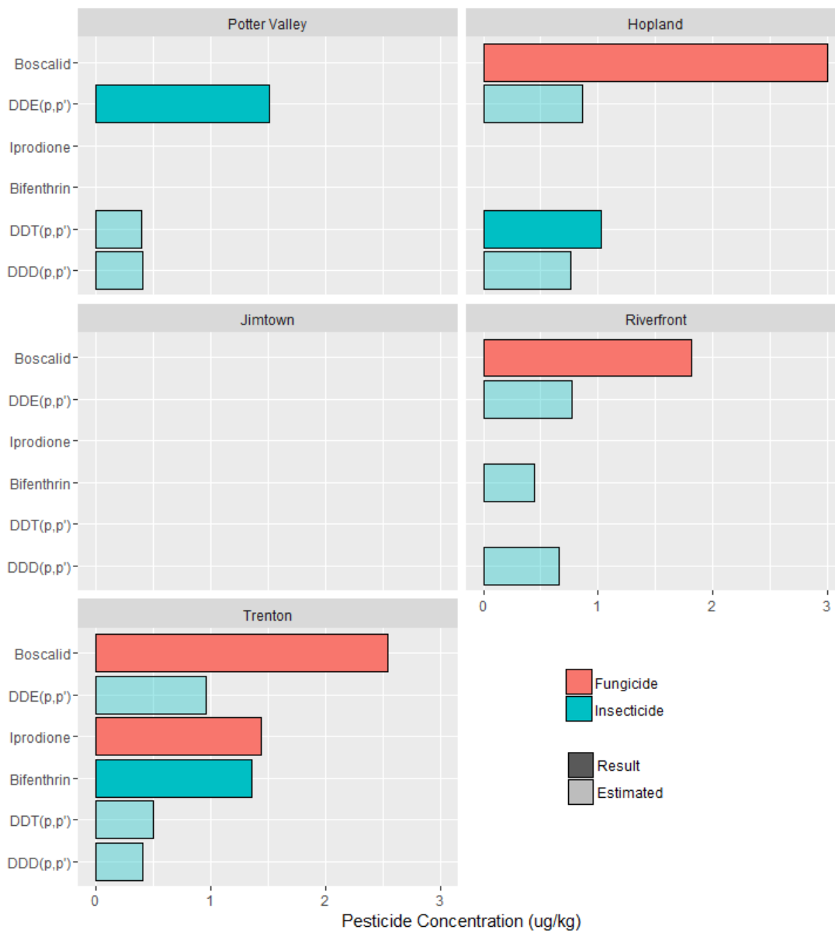
Figure 3-4A. Sediment results (µg/kg) by location – detected analytes
