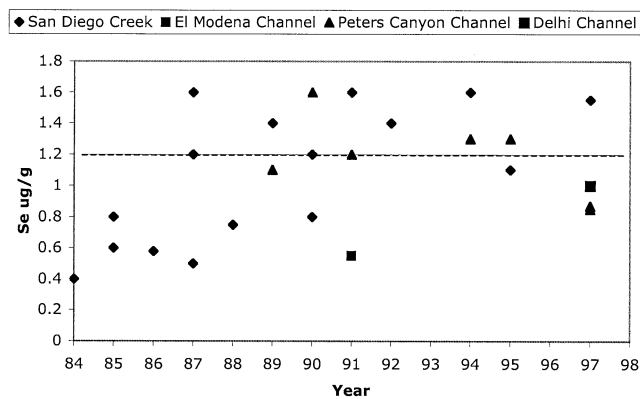
Fig. 1. Whole-body concentrations of Se in red shiner ( N. utrensis ) collected from San Diego Creek and other channels in the Newport Bay watershed (data from CRWQCB 2001). Dashed line represents growth LOEC determined in the current study (1.2 \mu\text{g/g} wet weight).
