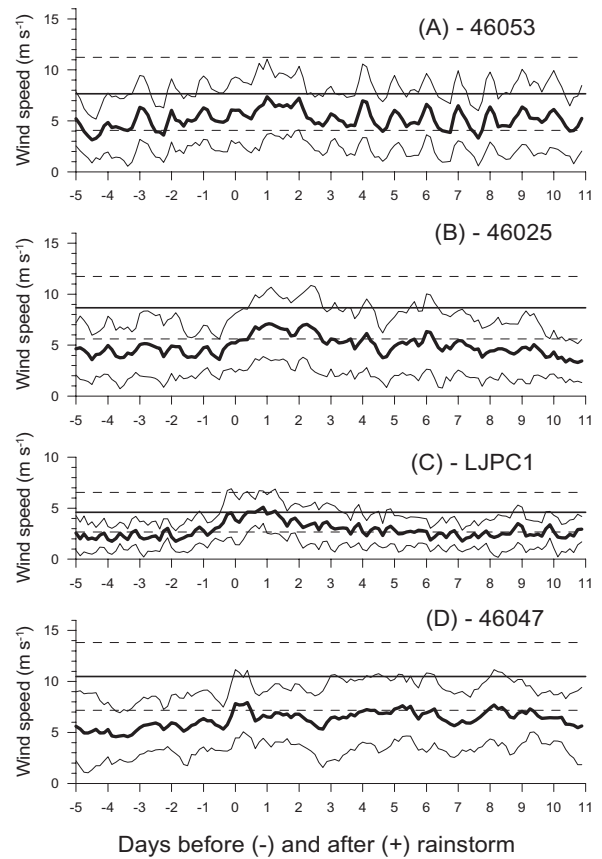
Figure 5. Absolute wind speed averaged for 3-hour periods from 5 days before rainstorm to ten days after rainstorm. Thick line indicates mean for each 3-hour period, thin lines indicate mean \pm standard deviation (SD). Horizontal lines indicate the values averaged for the days when the boat trips were weathered out (mean \pm SD).
