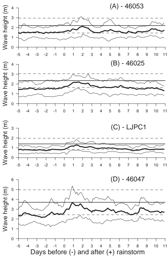
Figure 4. Absolute wave height averaged for 3-hour periods from 5 days before rainstorm to ten days after rainstorm. Thick line indicates mean for each 3-hour period, thin lines indicate mean \pm standard deviation (SD). Horizontal lines indicate the values averaged for the days when the boat trips were weathered out (mean \pm SD).
