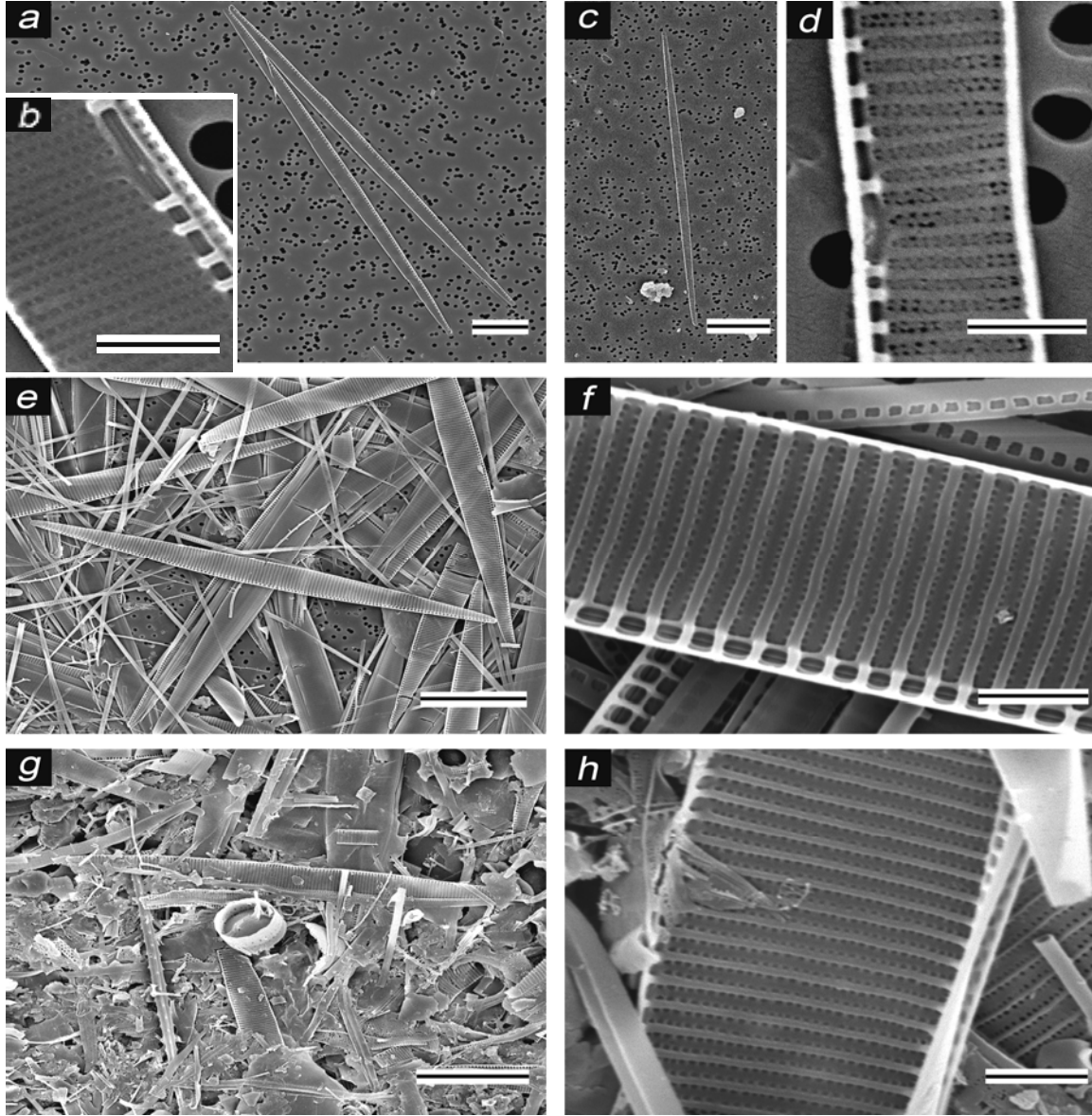
Fig. 4: Scanning electron micrographs of Pseudo-nitzschia spp. from the San Pedro Shelf area. a) P. cf. cuspidata cultured during spring 2003. Scale bar = 10 \mu\text{m} . b) Detail of P. cf. cuspidata showing central area of the valve. Scale bar = 2 \mu\text{m} . c) P. delicatissima from a natural sample collected during March 2004. Scale bar = 10 \mu\text{m} . d) Detail of central area of P. delicatissima valve in c. Scale bar = 1 \mu\text{m} . e) P. australis from a natural sample collected February 2004. Scale bar = 20 \mu\text{m} . f) Detail of P. australis valve in e. Scale bar = 1 \mu\text{m} . g) P. australis from a sediment trap sample collected April 16 - 22 from 500m depth in the San Pedro Channel. Scale bar = 20 \mu\text{m} . h) Detail of P. australis valve in g. Scale bar = 2 \mu\text{m} .
