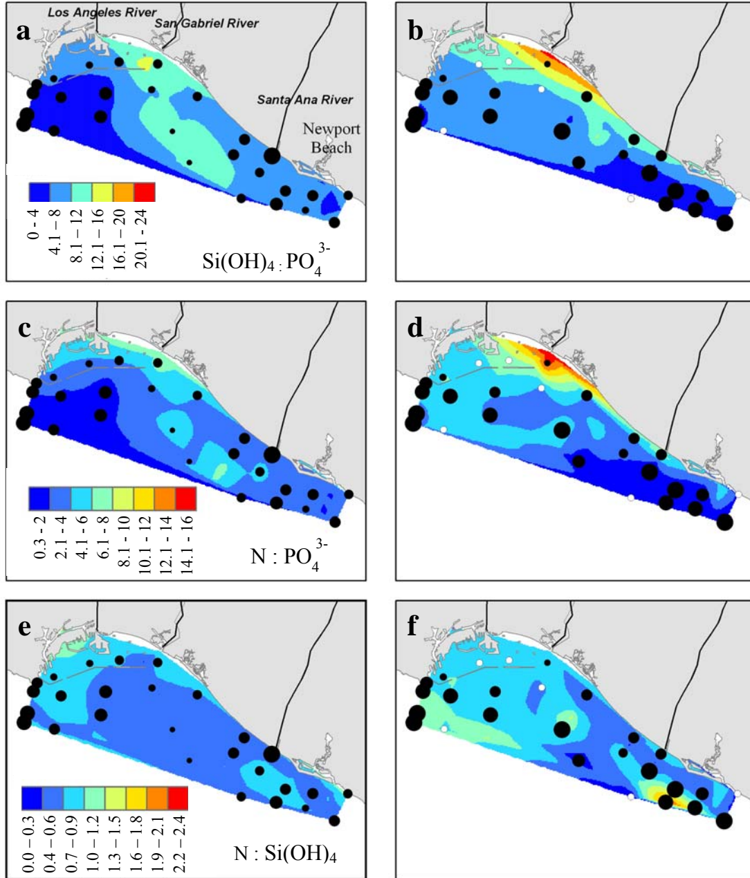
Fig. 8: Nutrient ratios ( \text{Si(OH)}_4 : \text{PO}_4^{3-} , \text{N} : \text{PO}_4^{3-} and \text{N} : \text{Si(OH)}_4 ) in surface waters on February 27/28 (a,c,e) and March 1 (b,d,f), 2004. Cellular DA concentrations for each of the sampling stations are indicated by filled circles. Cellular DA could not be calculated for sampling stations where Pseudo-nitzschia abundances or particulate DA concentrations were below the limit of detection (empty circles).
