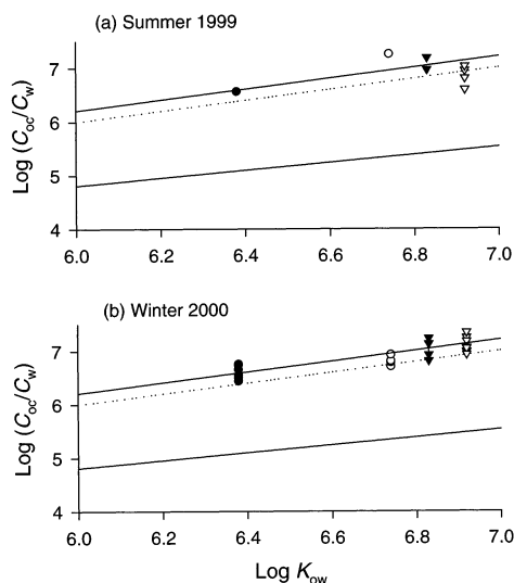
FIGURE 4. Partition coefficients of PCBs 101 (●), 118 (○), 138 (▼), and 153 (▽) between the suspended solid phase and the dissolved phase in water column samples collected during (a) summer 1999 and (b) winter 2000. The upper and lower solid lines represent the empirical \log K_{oc} values proposed by Karichhoff et al. (14) and Schwarzenbach and Westall (15), respectively. The dotted line is the \log K_{ow} - \log K_{ow} correlation.
