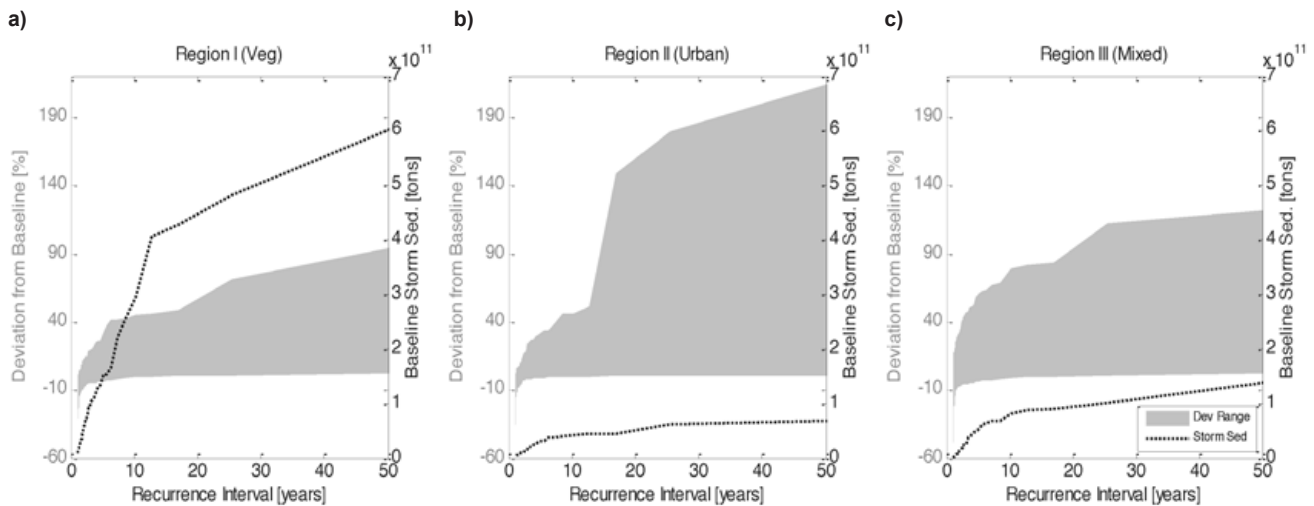
Figure 8. Recurrence interval of annual storm sediments due temperature increase and precipitation variability. Left axis corresponds to the range in percent deviation (shaded area) in storm sediments. Right axis corresponds to the baseline simulation of storm sediments (dotted line) for Region I, Region II, and Region III.
