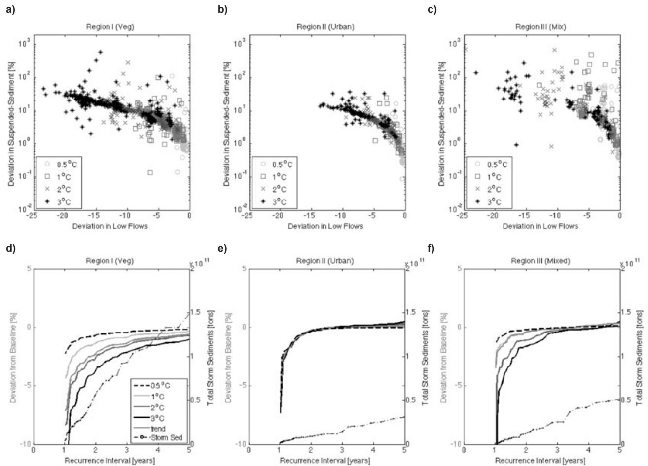
Figure 7. Percent deviation in daily suspended-sediment versus percent deviation in daily low-flow (a - c) and recurrence interval of annual storm sediments due temperature increase during low flow (d - f). Low flow corresponds to 90% probability of exceedance.
