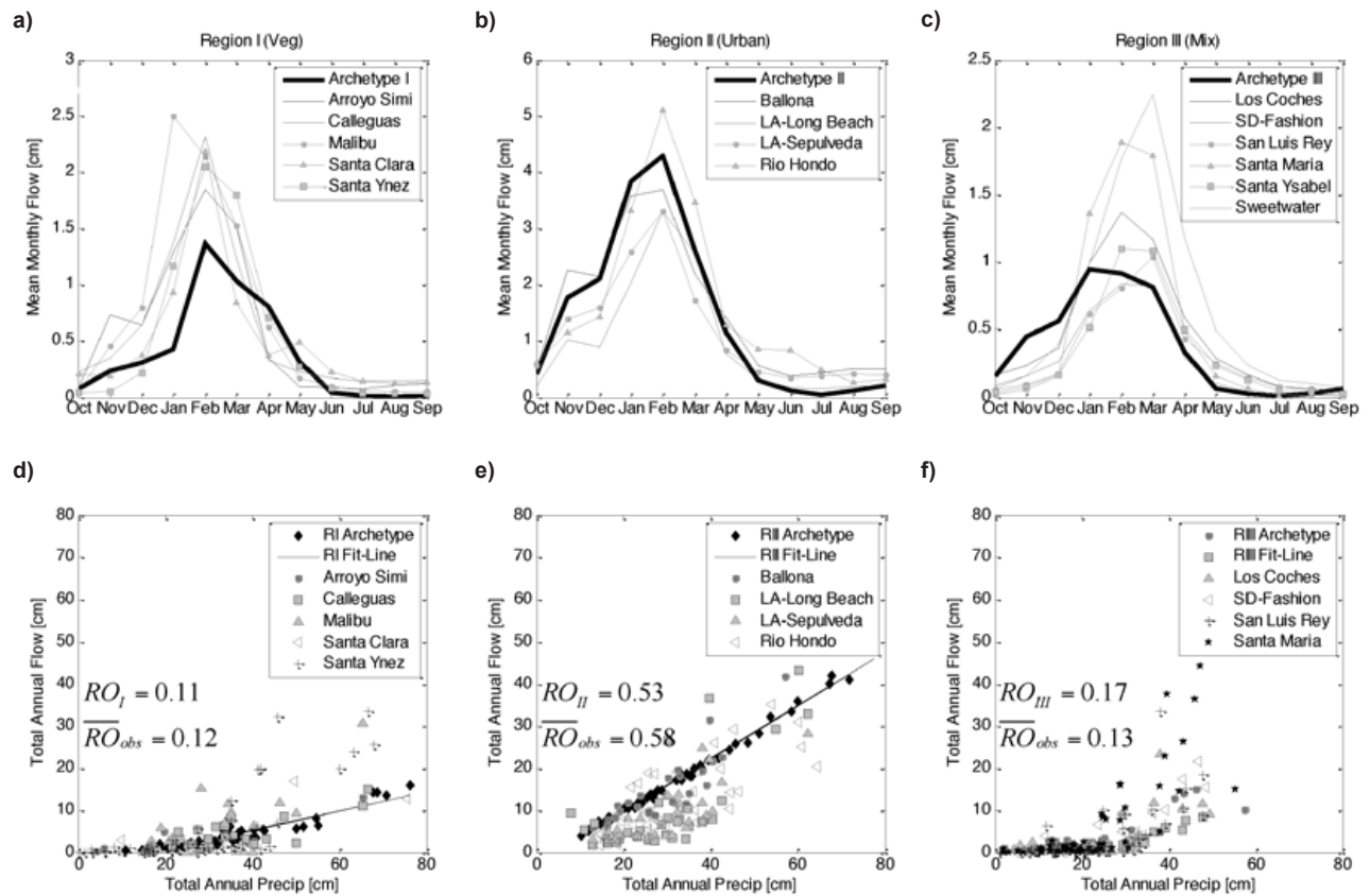
Figure 3. Archetypal comparisons of mean monthly flow behavior (a – c) and total annual flow versus annual precipitation (d – f) for each respective region.
