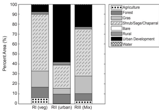
Figure 1. Percent of total area of aggregated land-cover distributions for Regions I through III.
