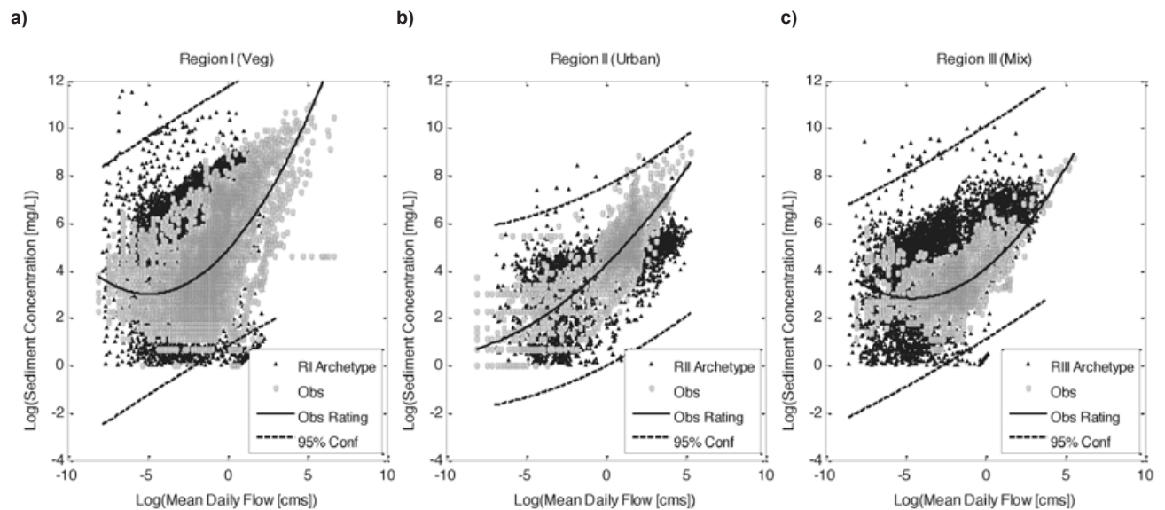
Figure 4. Solid lines are the log(Suspended-sediment) rating curves (2nd order) for observed sites within Region I, Region II, and Region III. Dashed lines are the \pm 95\% confidence intervals for the simulated log (suspended-sediment) rating curves.
