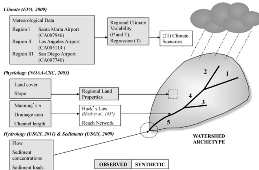
Figure 2. Methodology for development of regional watershed archetypes. Shaded boxes indicate the usage of observed meteorological, land cover and hydrologic data (sources listed); non-shaded boxes indicate the usage of empirical and/or synthetic approaches.
