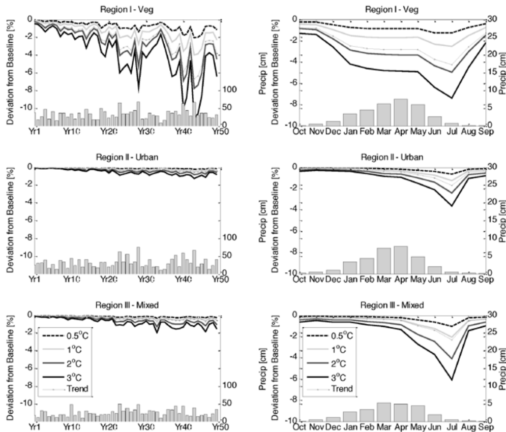
Figure 5. Percent change in total annual flow and mean monthly flow from baseline simulations for the 50-year increasing temperature scenarios only. The bottom bar graphs are the total annual precipitation and mean monthly precipitation used for each region. These temperature increase scenarios had no change in baseline precipitation.
